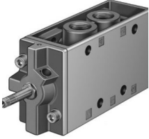
9440408887 MFH-5-1/2 Solenoid valve
