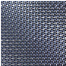
941222687 Wire Mesh For Stone Separator Mesh Size 1.20mm Wire Ø0.8mm Width 140Cm
