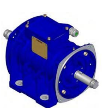
941242687 Vibro Motor SPV 4.0 0,55 kW 600 rpm without Counter Weights & Covers
