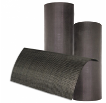
943102887 Wire Mesh for Wheat Scourer Mesh Size:1.80 mm Wire Q:1.5 mm Thickness:2 mm Width: 1 m
